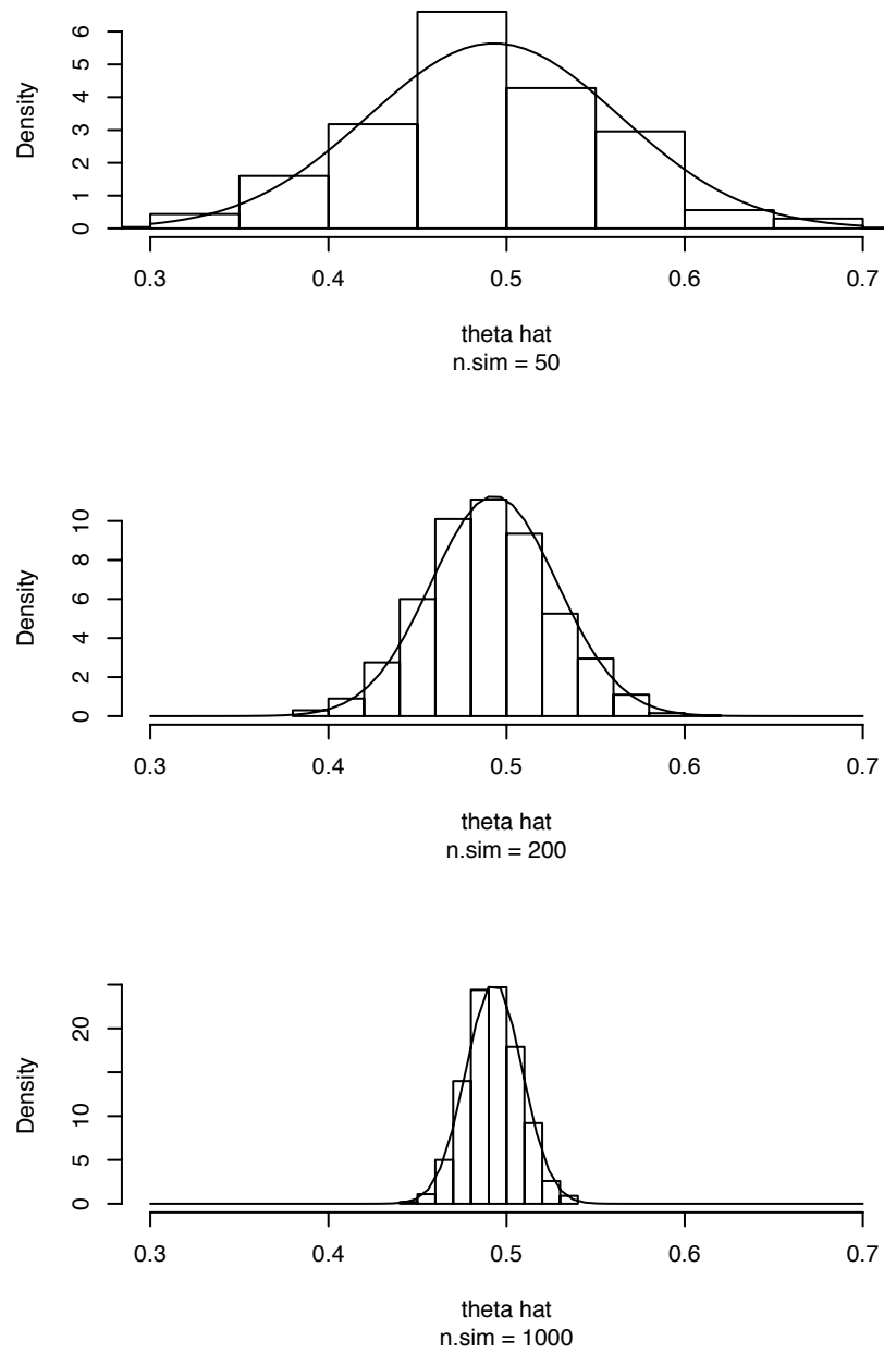
Figure 1.23: Histograms of craps simulations. Solid curves are Normal approximations according to the Central Limit Theorem.
